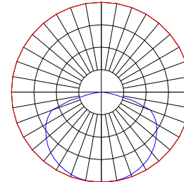
RPL-6GD Polar Curves
