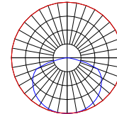
RPL-6GD Polar Curves
