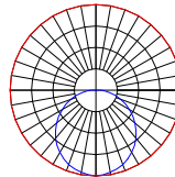
RPL-6FD Polar Curves
