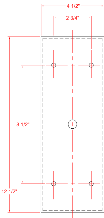
MOUNTING DETAIL MODIFIED TO MATCH EXISTING
