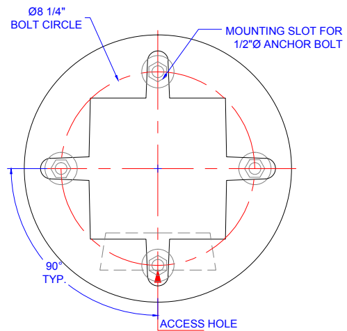
MOUNTING DETAIL
