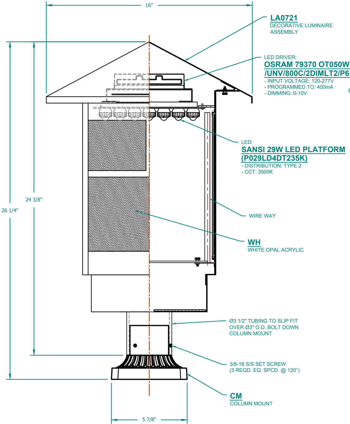
MOUNTING DETAIL
